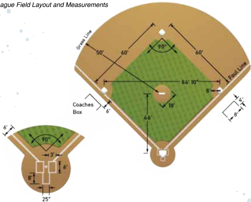
Little League Field Layout and Measurements
